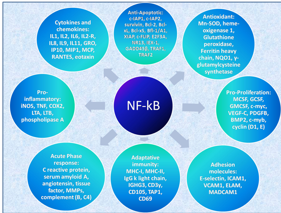
Fig. 3. Overview of the different groups of genes and molecules that have NF-kB response elements. In principle these could be activated by NF-kB signaling pathway triggered by the ROS produced during LLLT.
